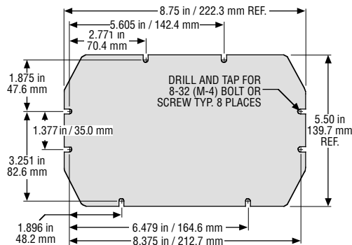
ENCLOSURE DIMENSIONS
