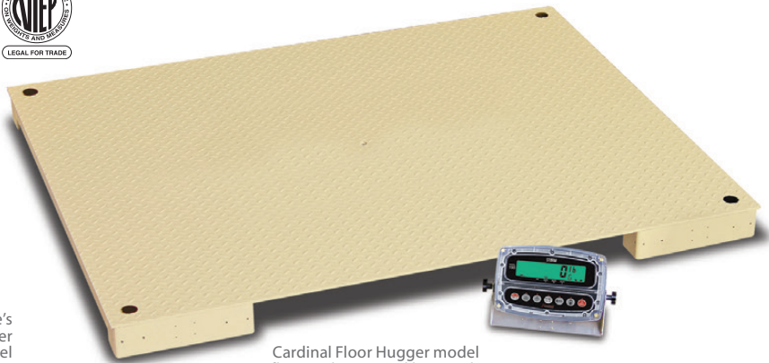
Cardinal Floor Hugger model FHN-1054 floor scale pictured here with optional model 190 digital weight indicator
