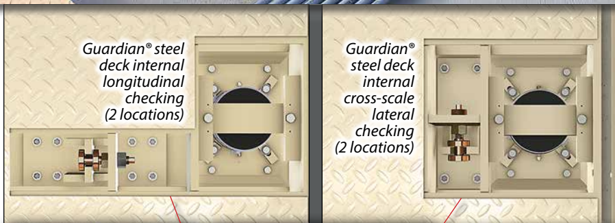
Overhead view of a 70-ft-long steel deck ARMOR® truck scale with Guardian® hydraulic load cells (checking access covers removed)
