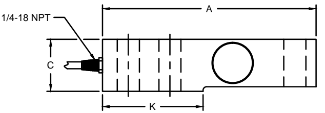
CG-23-SSW-1 NON-THREADED LOAD HOLE
