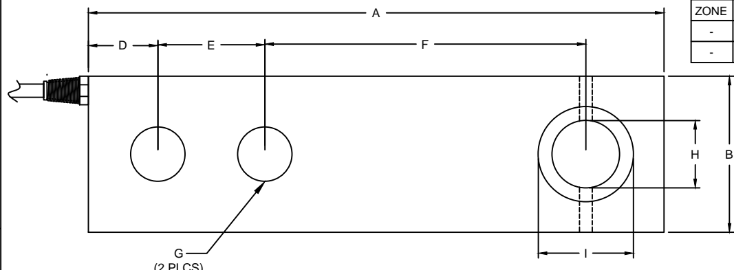
CG-745 TOP VIEW
